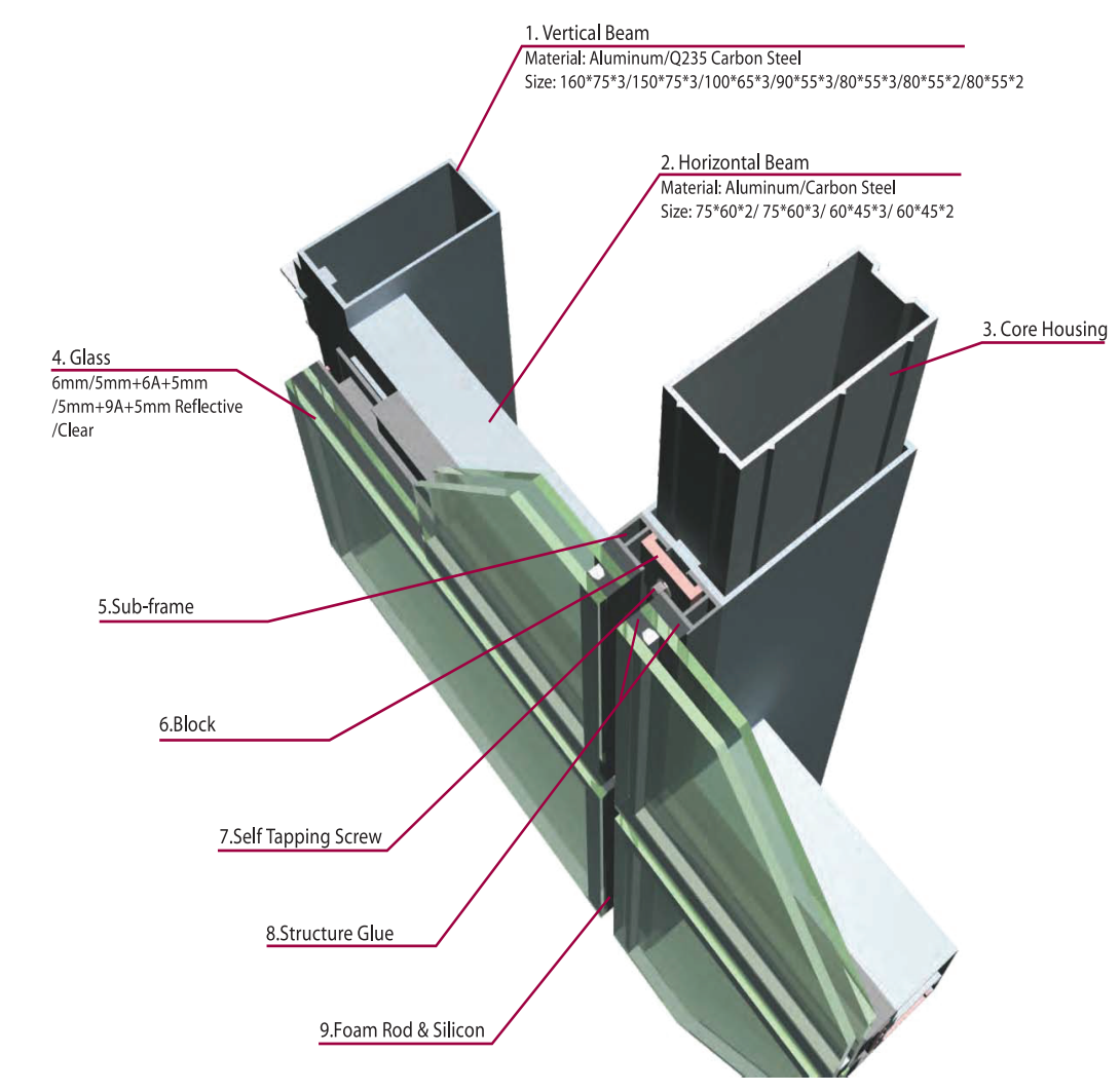
Semi Exposed Frame glass curtain wall
